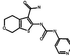
Compound B73
