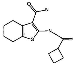
Compound D9
