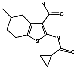
Compound D37
