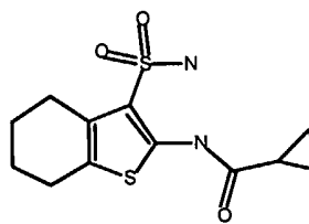
Compound D86
