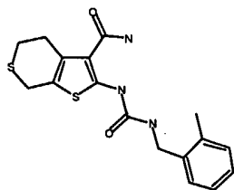
Compound C33
