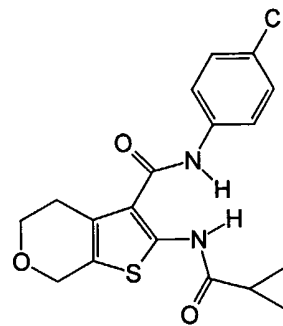
Compound B248
