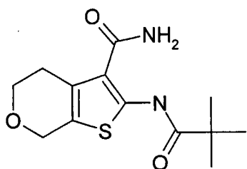
Compound B18
