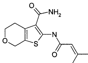
Compound B17
